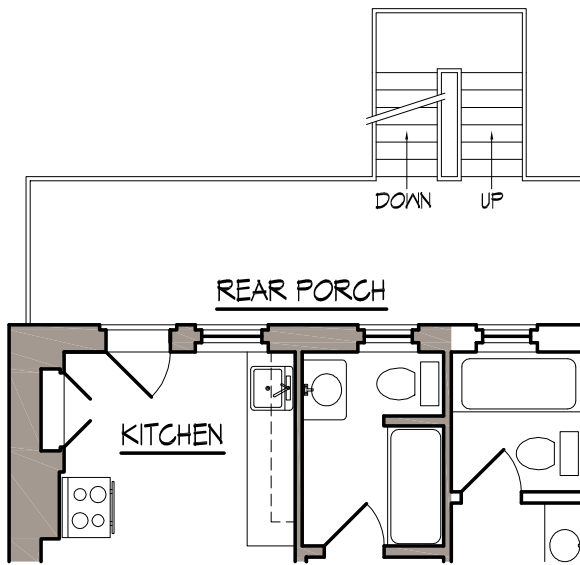
SECOND FLOOR REAR PORCH PLAN
