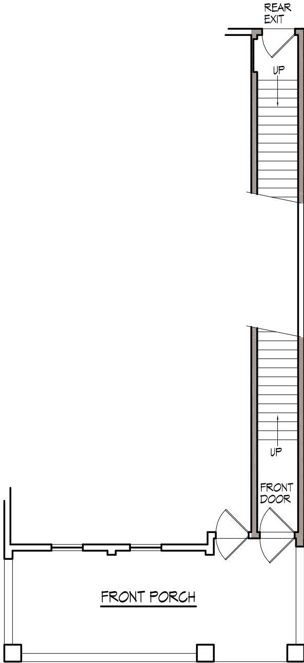
FIRST FLOOR ENTRY HALL PLAN
